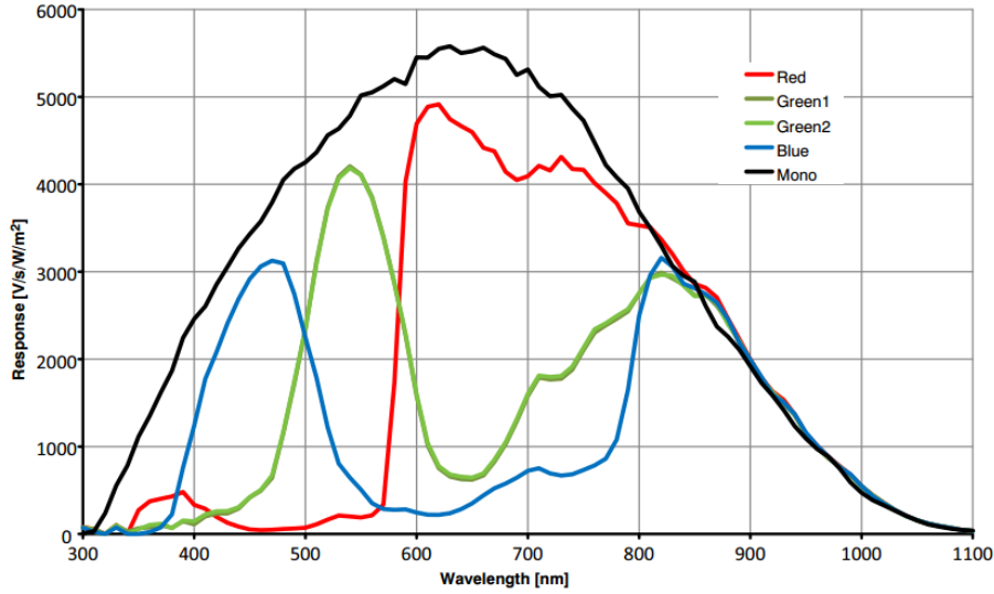
Figure 4-26 MER-131-75GC / MER-131-75GM sensor spectral response
