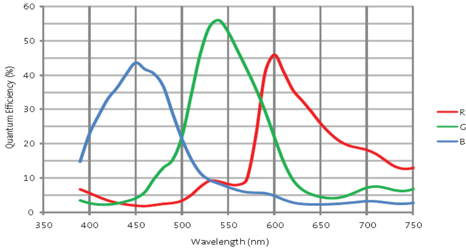
Figure 4-80 MER-1520-7GC sensor spectral response
