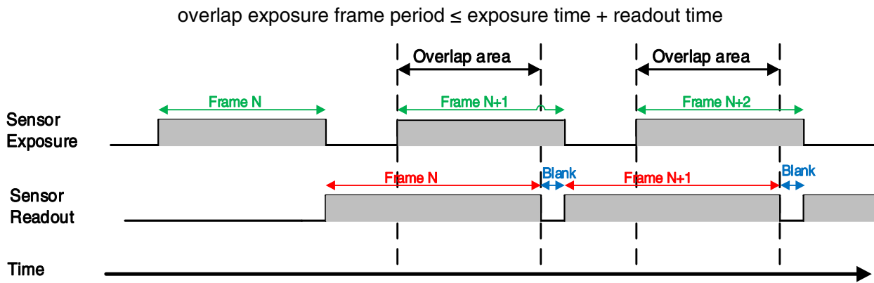
Figure 8-16 The exposure sequence diagram in overlap exposure mode
