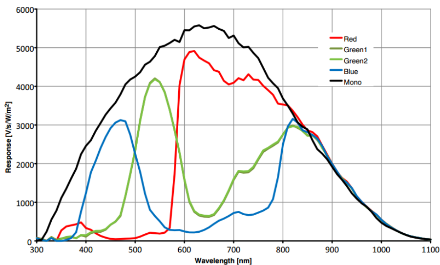
Figure 4-27 MER-131-75GC-P / MER-131-75GM-P sensor spectral response
