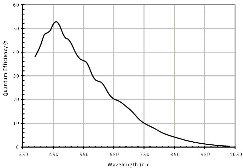
Figure 4-75 MER-1070-10GM-P sensor spectral response
