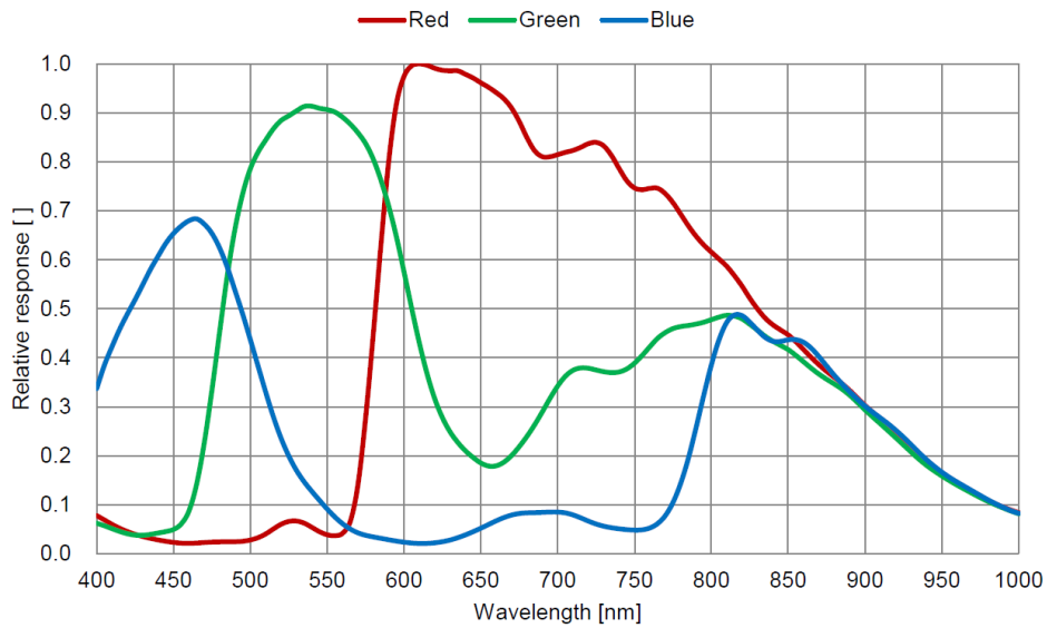
Figure 4-14 MER-041-302GC-P sensor spectral response
