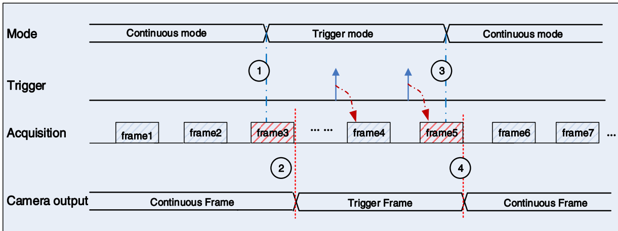
Figure 8-9 Switch acquisition mode during reading out
