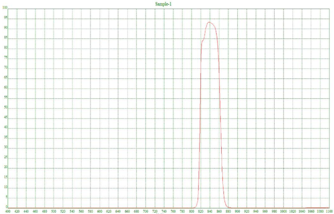
Figure 6-3 Visible light cut-off filter transmittance curve for MER-203-30GC-P-L-F03
