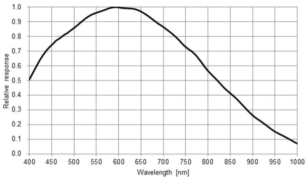
Figure 4-61 MER-503-20GM sensor spectral response
