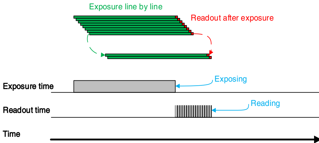
Figure 8-13 Electronic rolling shutter
