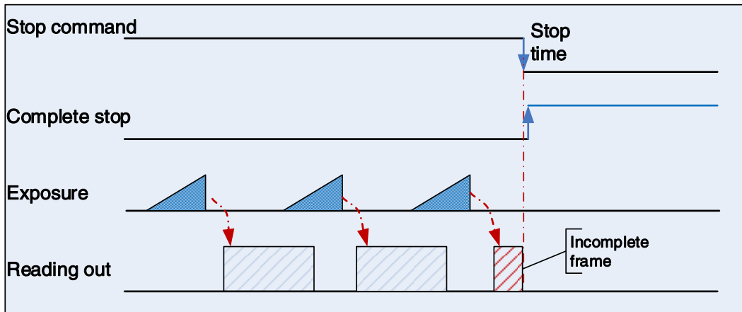
Figure 8-7 Acquisition stop during reading out
