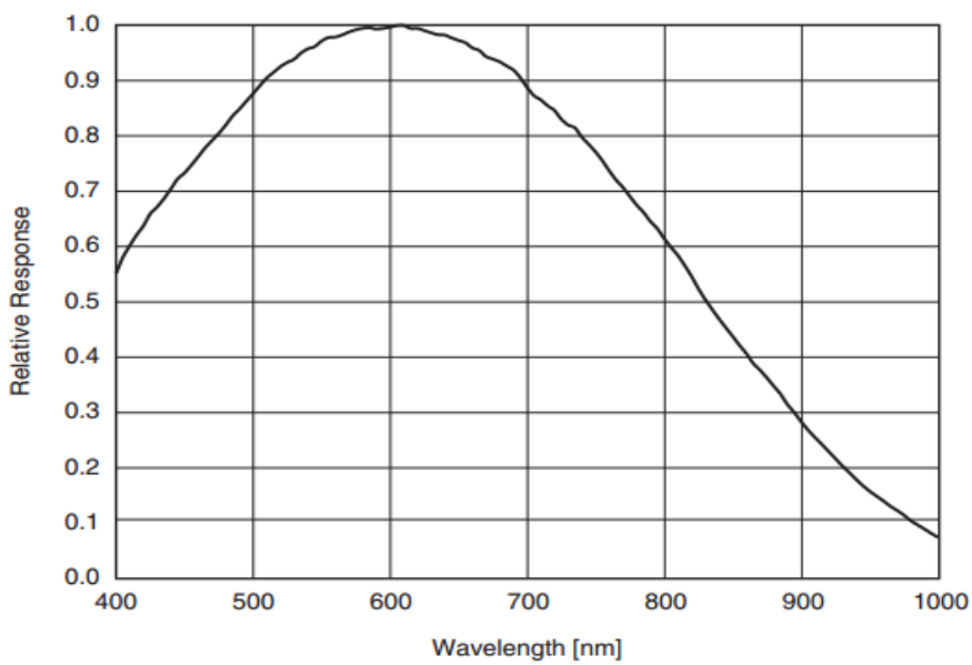
Figure 4-4 MER-030-120GM-P sensor spectral response
