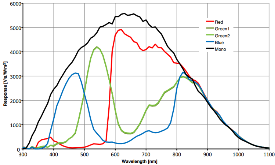
Figure 4-5 MER-031-300GC / MER-031-300GM sensor spectral response
