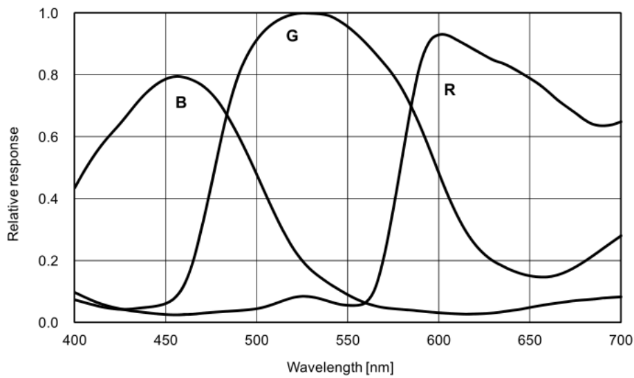
Figure 4-82 MER-2000-5GC sensor spectral response
