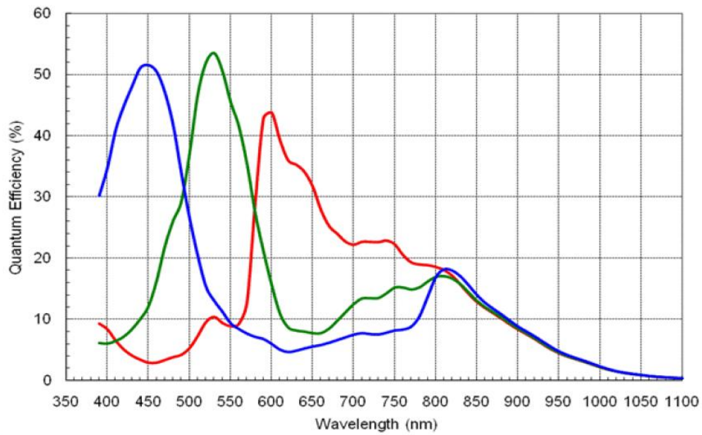
Figure 4-58 MER-500-14GC-P sensor spectral response
