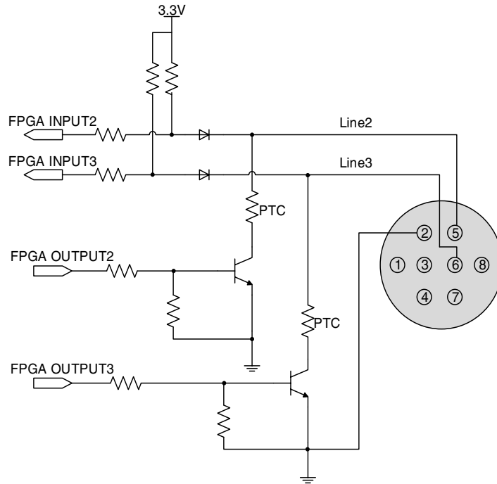
Figure 7-7 GPIO 2/3 (bidirectional) circuit
