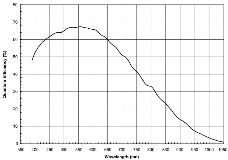
Figure 4-38 MER-133-54GM-P sensor spectral response
