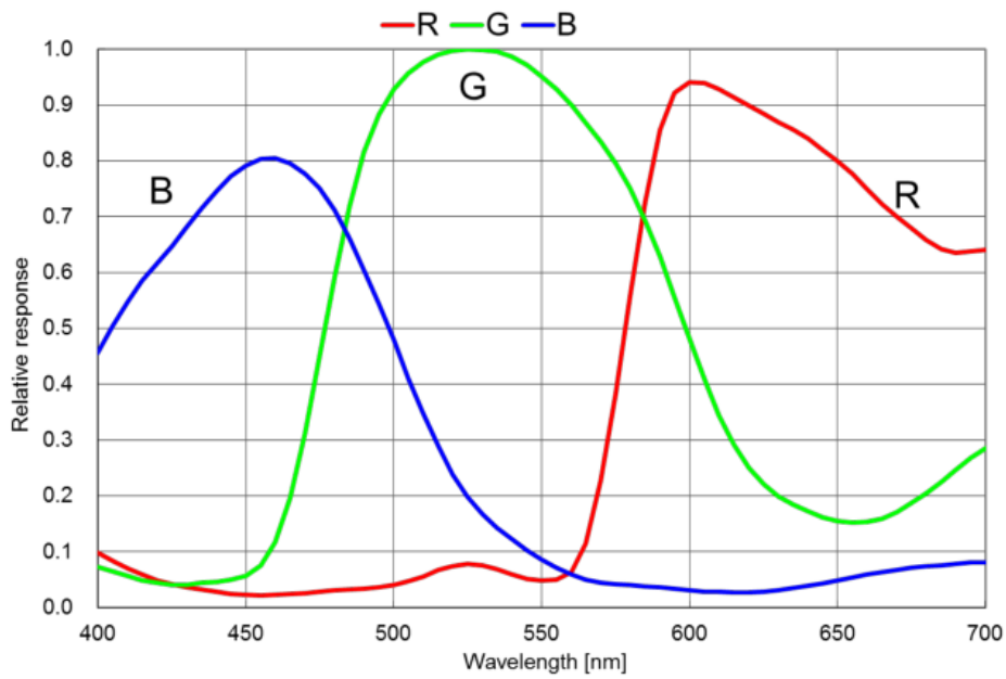
Figure 4-68 MER-630-16GC sensor spectral response
