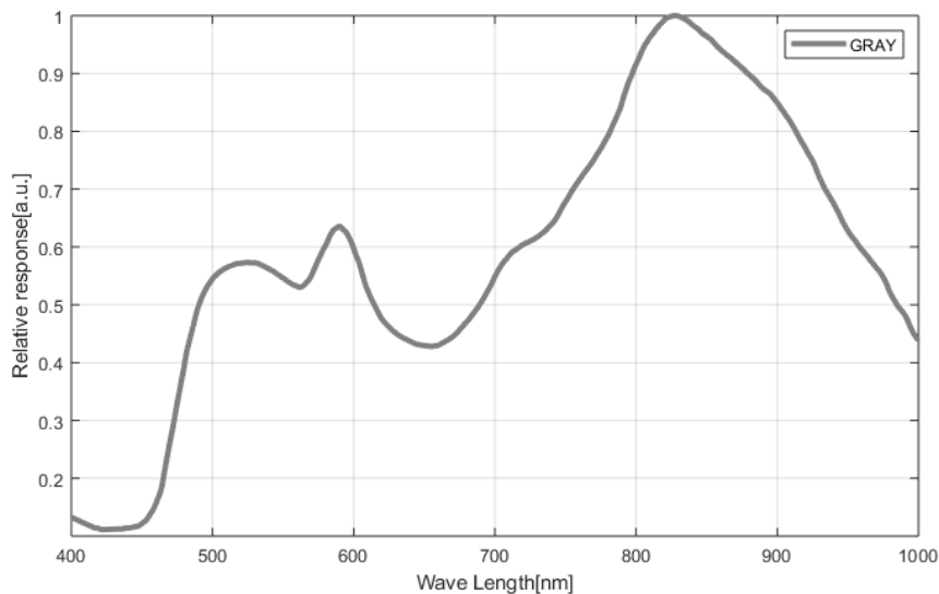
Figure 4-50 MER-204-30GC-P-L-F02 sensor spectral response
