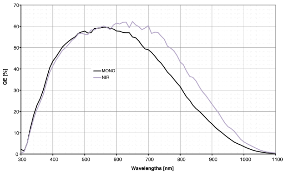
Figure 4-28 MER-131-75GM-P NIR sensor spectral response
