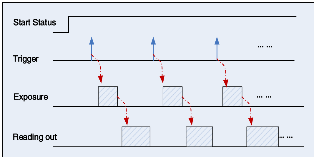
Figure 8-6 Trigger acquisition process
