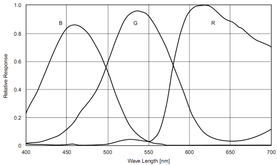
Figure 4-41 MER-200-20GC sensor spectral response
