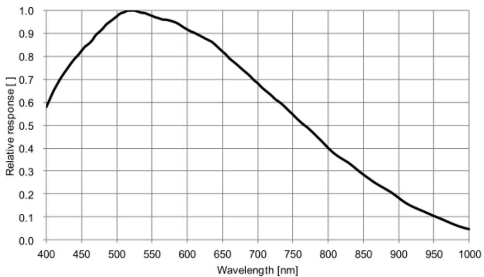
Figure 4-54 MER-231-41GM-P sensor spectral response
