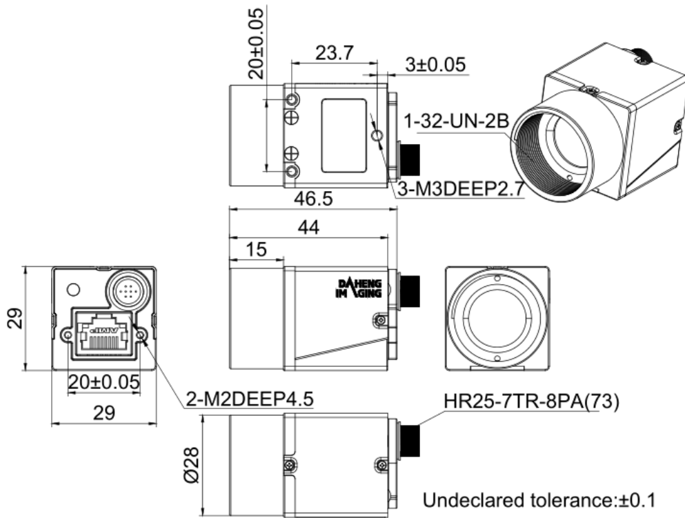
Figure 5-3 MER-G mechanical dimensions
