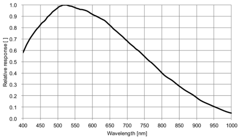
Figure 4-52 MER-231-41GM sensor spectral response
