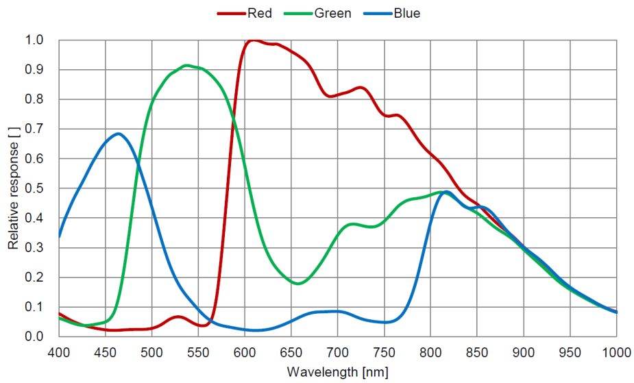
Figure 4-12 MER-041-302GC sensor spectral response
