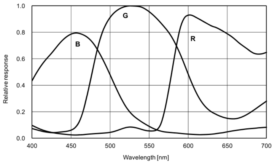
Figure 4-84 MER-2000-5GC-P sensor spectral response
