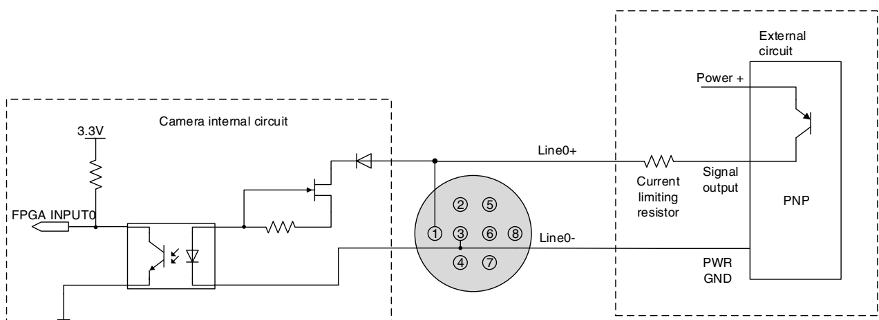
Figure 7-3 PNP photosensor connected to opto-isolated input circuit
