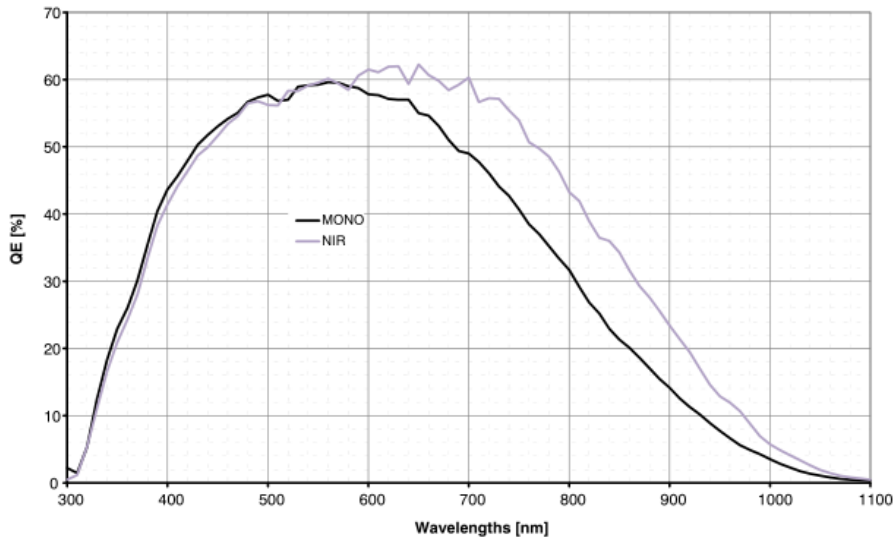
Figure 4-7 MER-031-300GM-P NIR sensor spectral response
