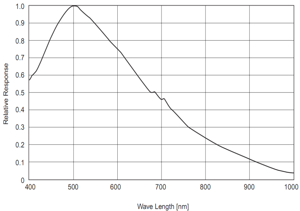
Figure 4-40 MER-200-14GM sensor spectral response
