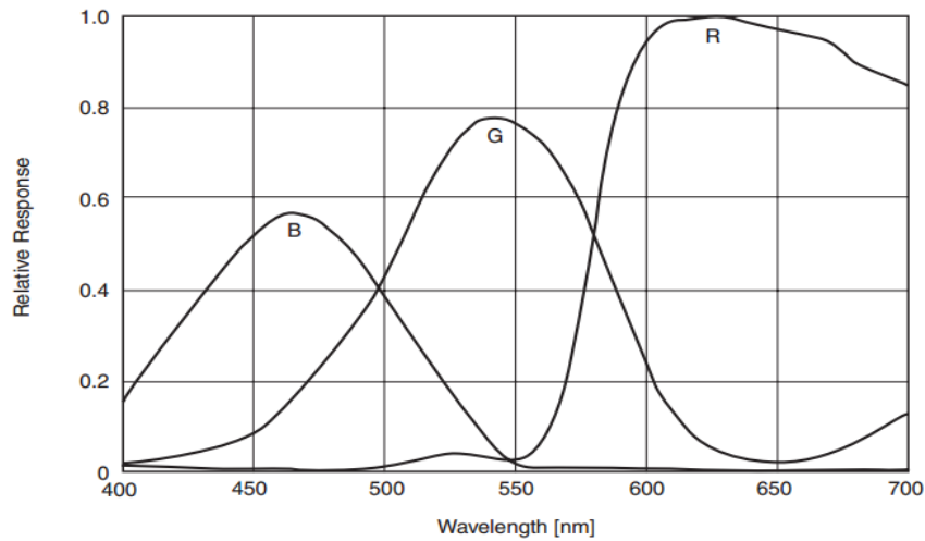
Figure 4-1 MER-030-120GC sensor spectral response
