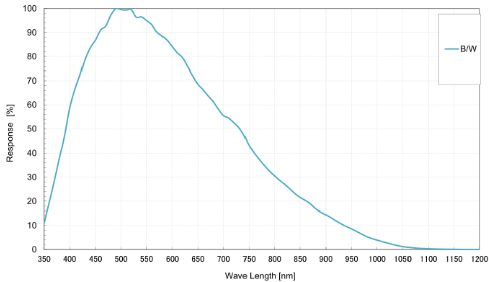
Figure 4-65 MER-504-10GM-P sensor spectral response
