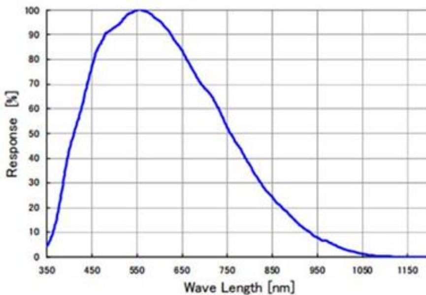
Figure 4-34 MER-132-43GM-P sensor spectral response
