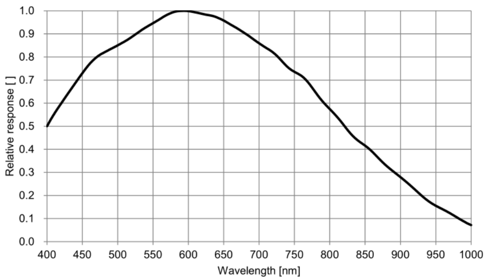
Figure 4-15 MER-041-302GM-P sensor spectral response
