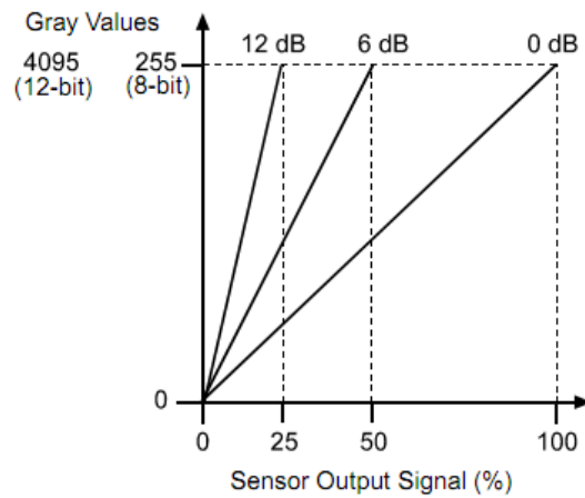
Figure 8-18 The camera's response curve
