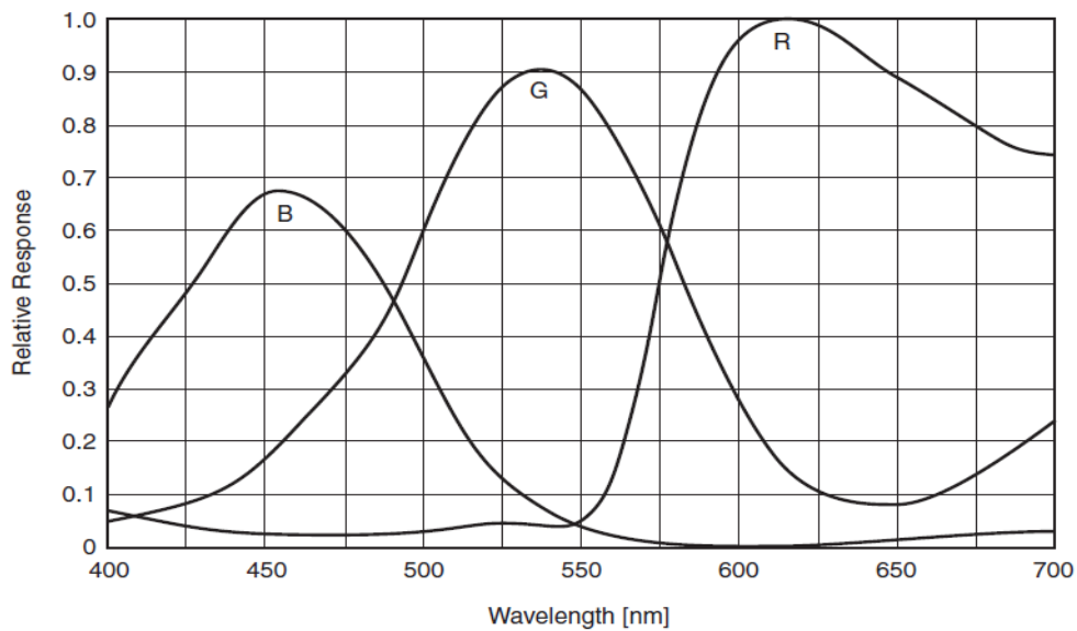
Figure 4-23 MER-125-30GC-P sensor spectral response
