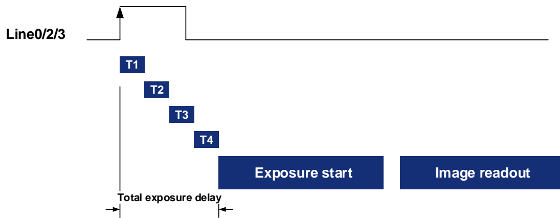
Figure 8-11 Exposure delay
