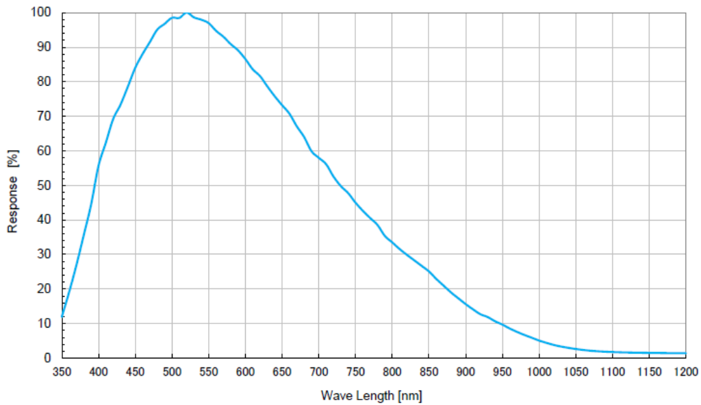
Figure 4-46 MER-201-25GM sensor spectral response
