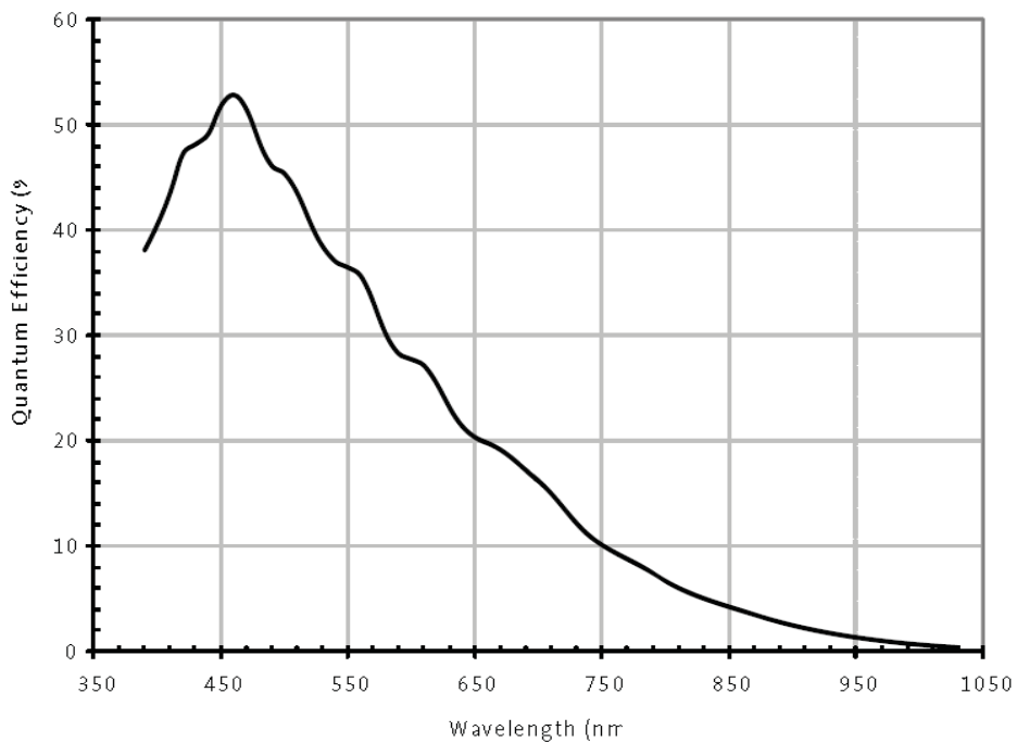
Figure 4-73 MER-1070-10GM sensor spectral response
