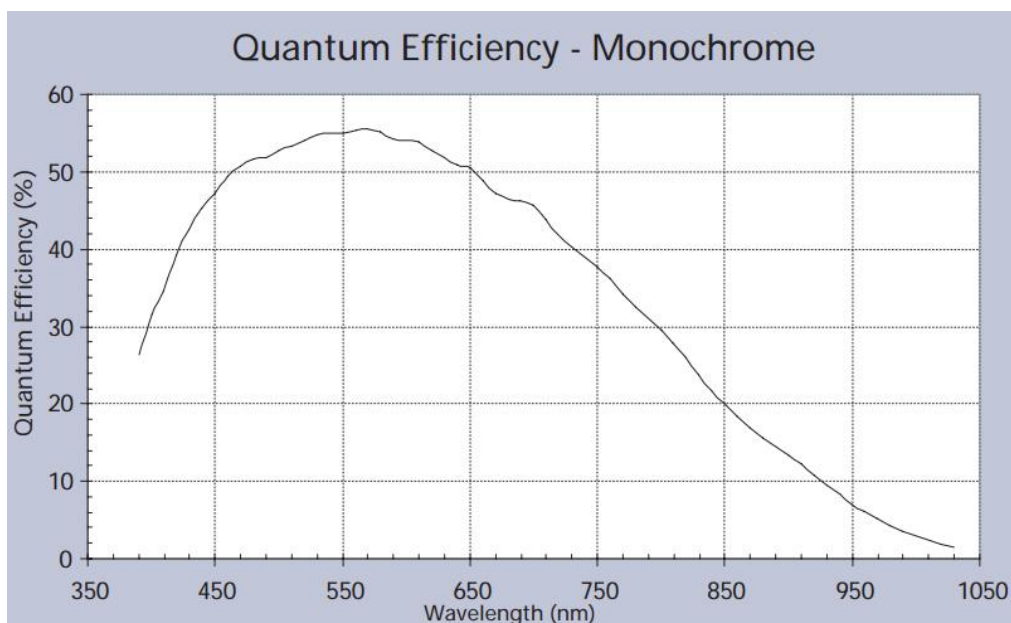
Figure 4-25 MER-130-30GM sensor spectral response
