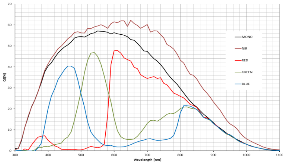
Figure 4-66 MER-530-20GM-P NIR sensor spectral response
