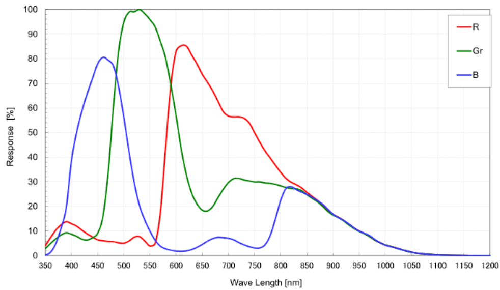
Figure 4-64 MER-504-10GC-P sensor spectral response
