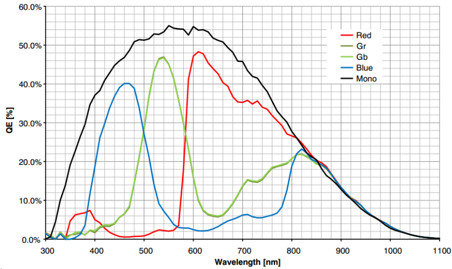
Figure 4-20 MER-051-120GC-P / MER-051-120GM-P sensor spectral response
