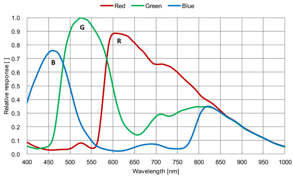
Figure 4-51 MER-231-41GC sensor spectral response
