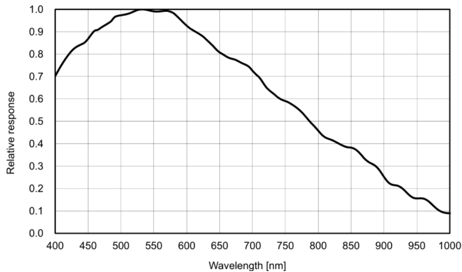
Figure 4-85 MER-2000-5GM-P sensor spectral response
