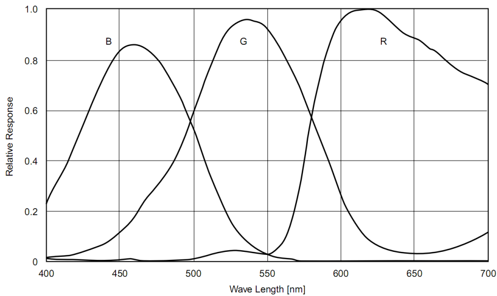
Figure 4-43 MER-200-20GC-P sensor spectral response
