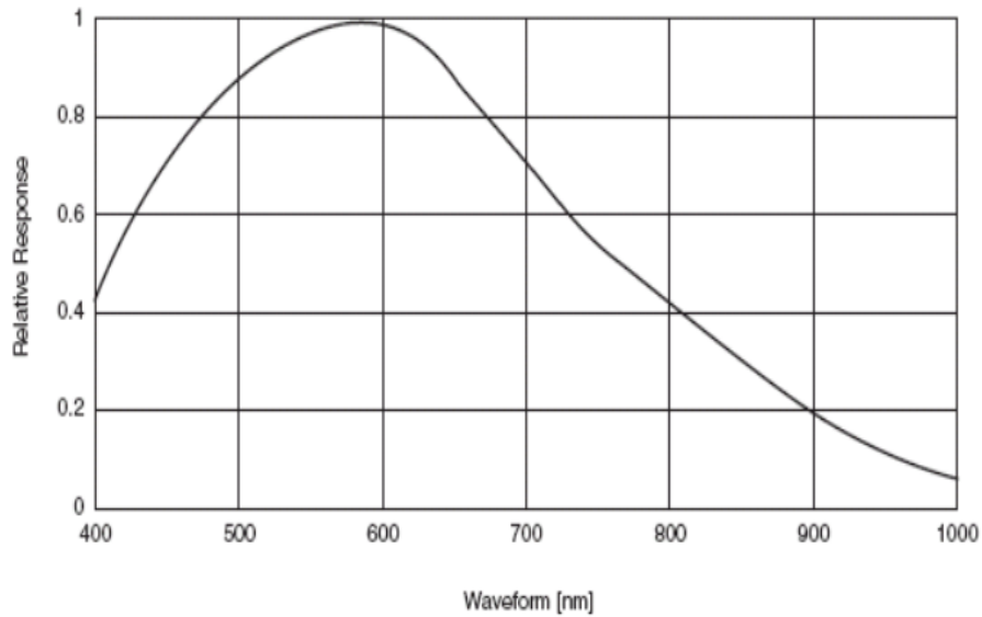
Figure 4-22 MER-125-30GM sensor spectral response
