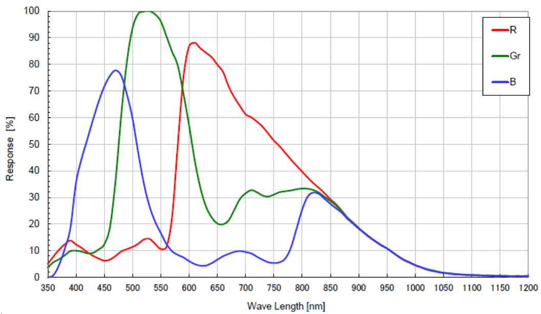
Figure 4-47 MER-201-25GC-P sensor spectral response
