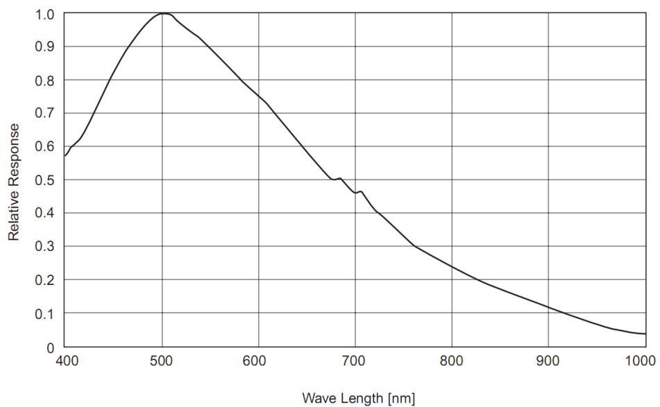
Figure 4-42 MER-200-20GM sensor spectral response
