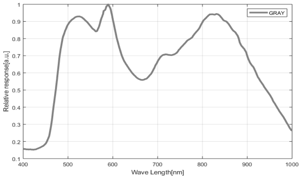
Figure 4-49 MER-203-30GC-P-L, MER-203-30GC-P-L-F03 sensor spectral response
