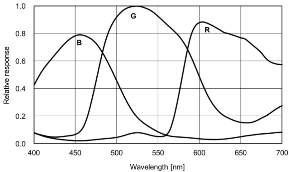
Figure 4-78 MER-1220-9GC-P sensor spectral response
