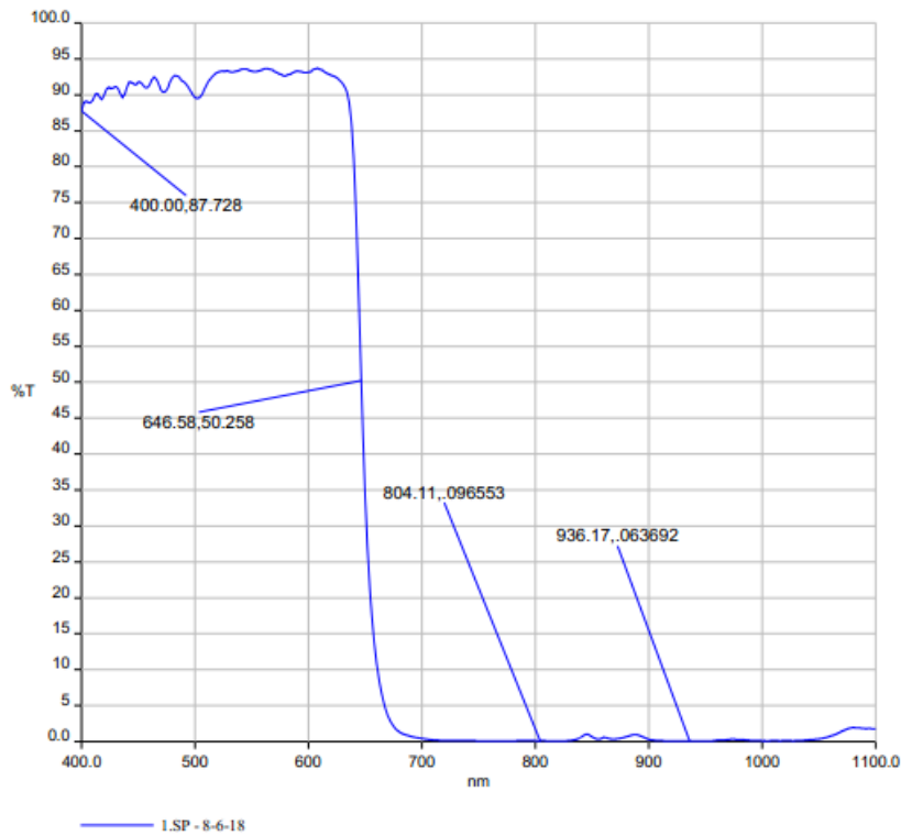
Figure 6-1 Infrared cut-off filter transmittance curve for MERCURY series color camera
