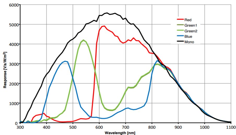
Figure 4-17 MER-050-200GC-P / MER-050-200GM-P sensor spectral response
