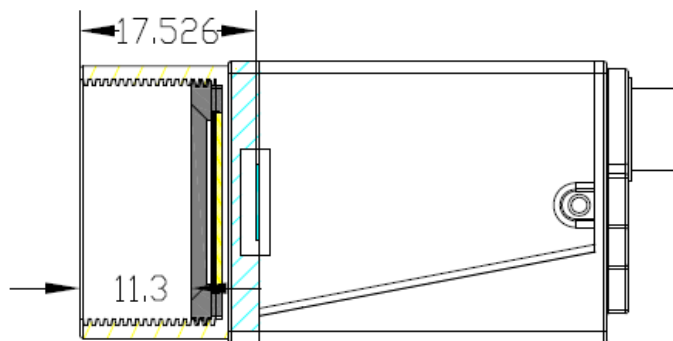
Figure 5-4 Optical interface of C-mount
