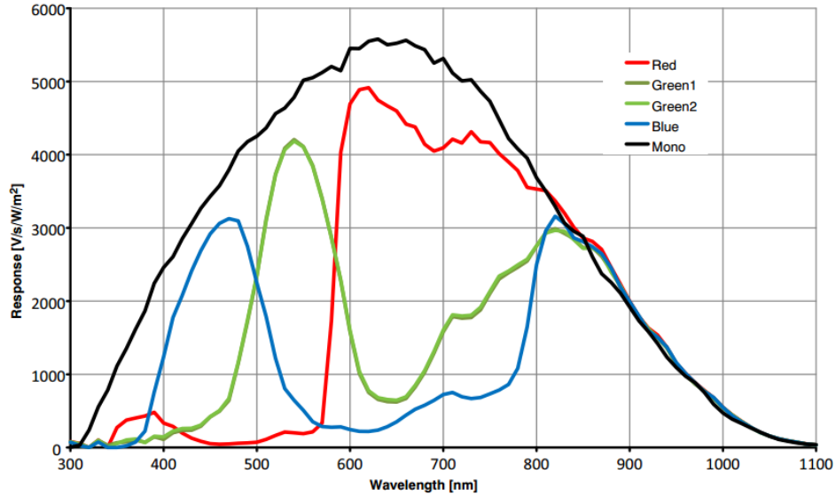
Figure 4-16 MER-050-200GC / MER-050-200GM sensor spectral response
