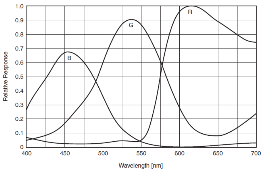
Figure 4-21 MER-125-30GC sensor spectral response
