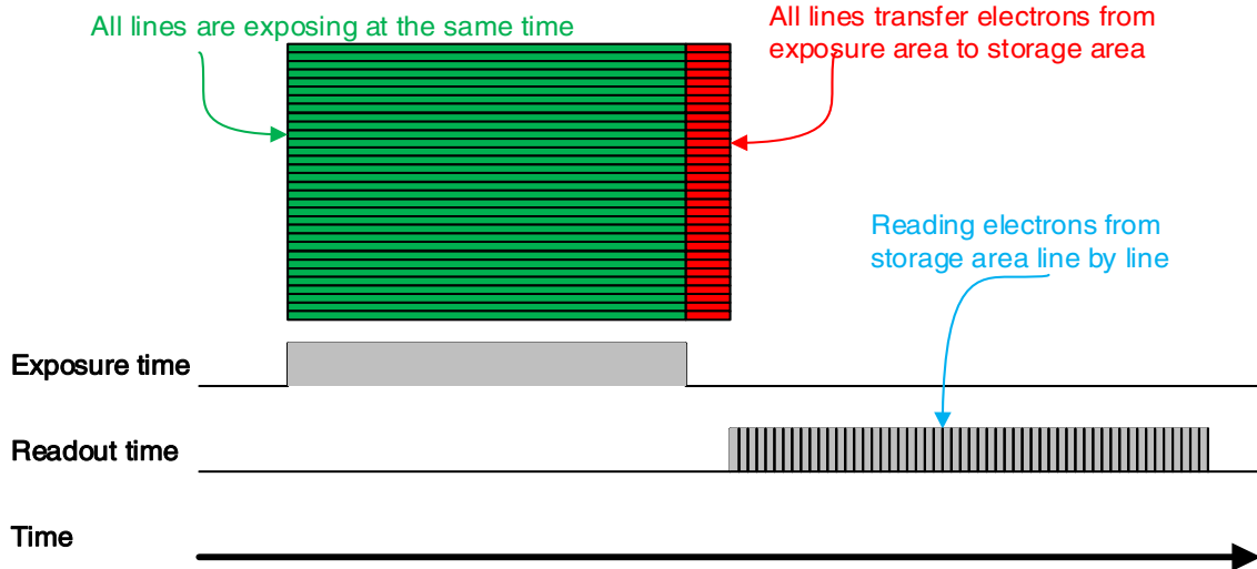
Figure 8-12 Global Shutter
