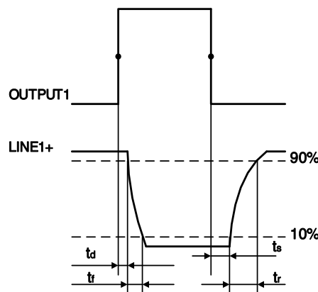
Figure 7-6 Parameter of opto-isolated output circuit
