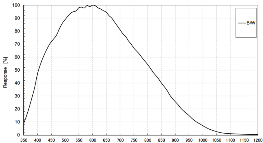
Figure 4-11 MER-032-120GM-P sensor spectral response
