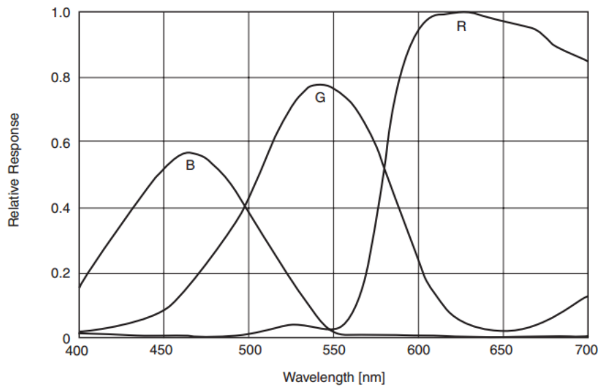
Figure 4-3 MER-030-120GC-P sensor spectral response
