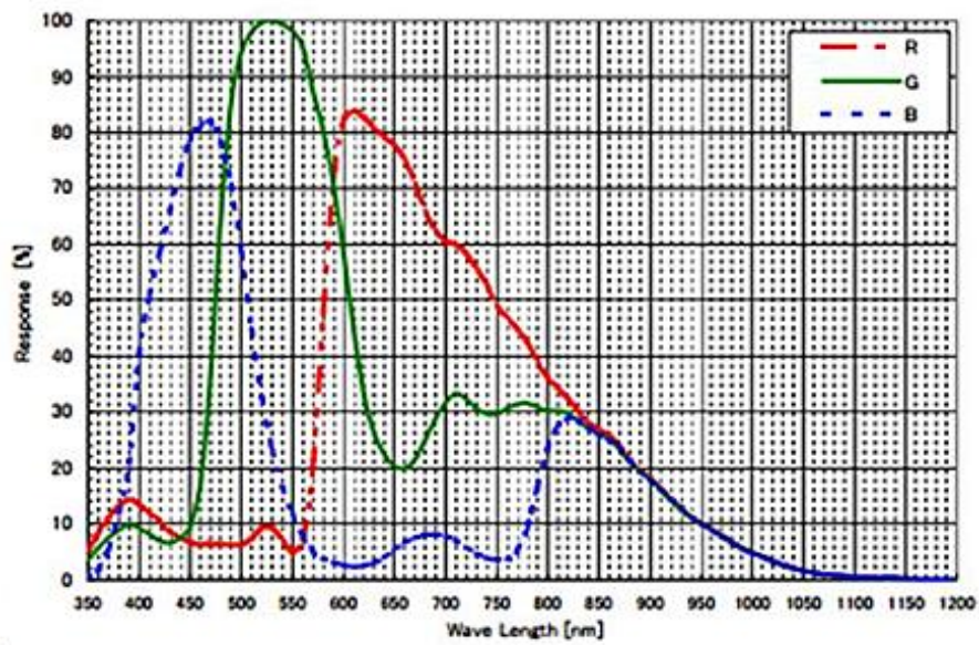
Figure 4-33 MER-132-43GC-P sensor spectral response
