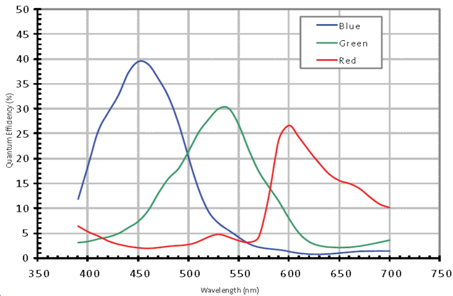
Figure 4-74 MER-1070-10GC-P sensor spectral response
