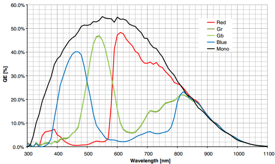
Figure 4-19 MER-051-120GC / MER-051-120GM sensor spectral response
