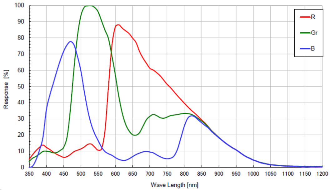
Figure 4-45 MER-201-25GC sensor spectral response
