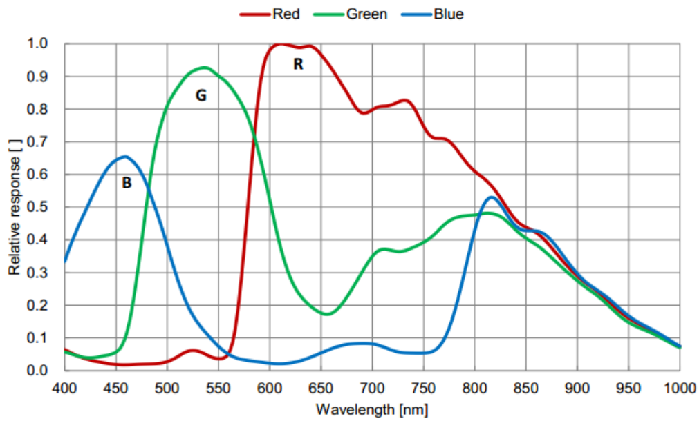
Figure 4-62 MER-503-20GC-P sensor spectral response
