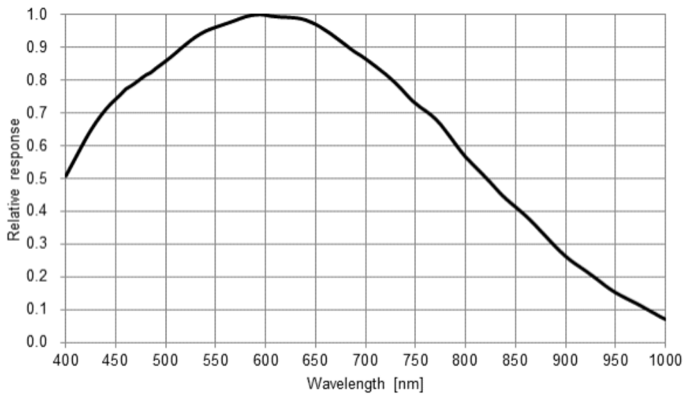
Figure 4-63 MER-503-20GM-P sensor spectral response
