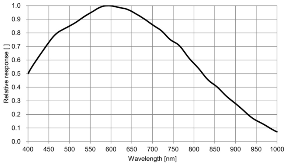
Figure 4-13 MER-041-302GM sensor spectral response
