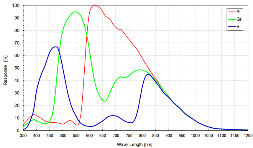
Figure 4-10 MER-032-120GC-P sensor spectral response
