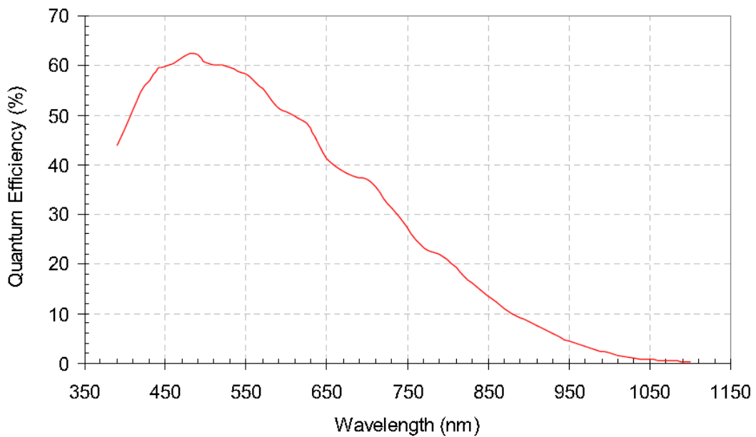
Figure 4-57 MER-500-14GM sensor spectral response
