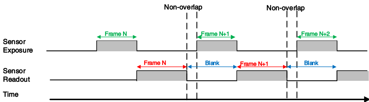
Figure 8-14 The exposure sequence diagram in non-overlap exposure mode
