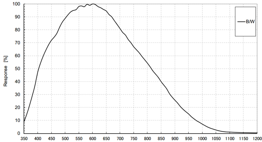
Figure 4-9 MER-032-120GM sensor spectral response
