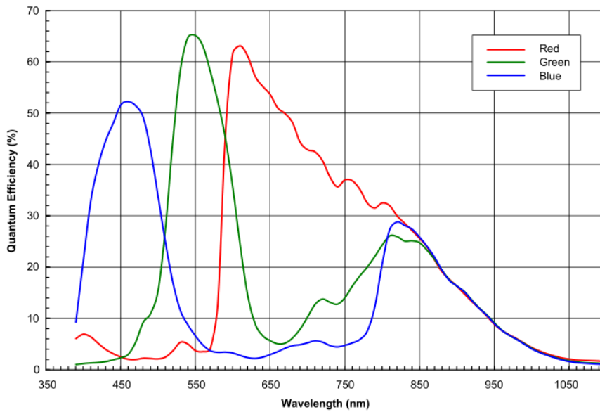
Figure 4-37 MER-133-54GC-P sensor spectral response
