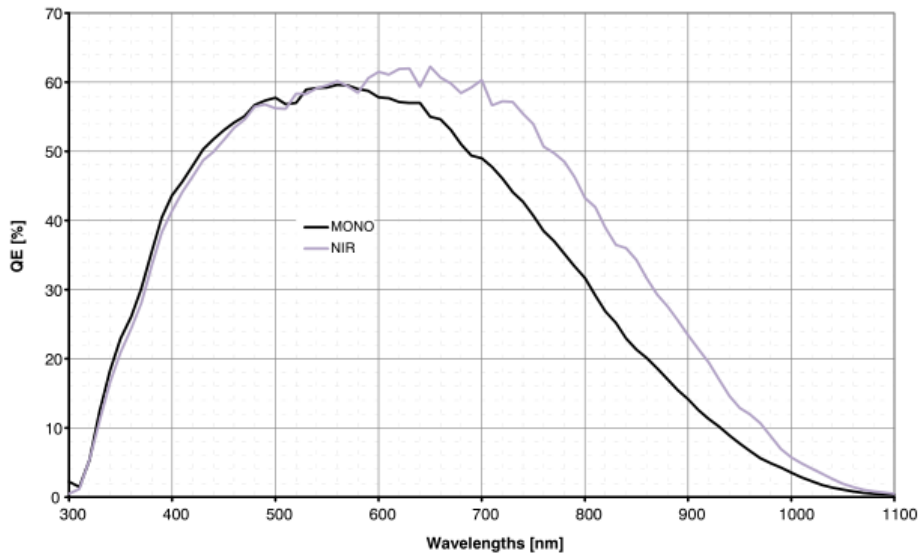
Figure 4-18 MER-050-200GM-P NIR sensor spectral response
