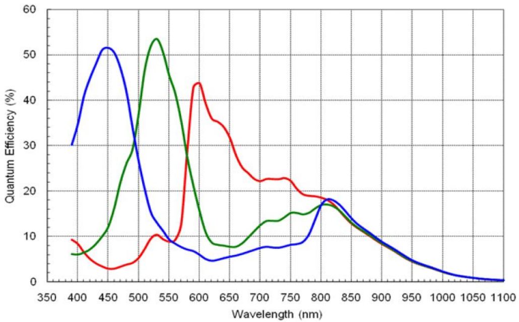
Figure 4-56 MER-500-14GC sensor spectral response
