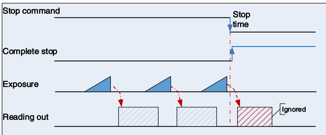
Figure 8-8 Acquisition stop during blanking
