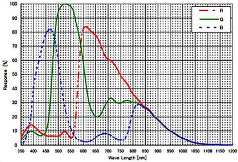
Figure 4-29 MER-132-30GC sensor spectral response
