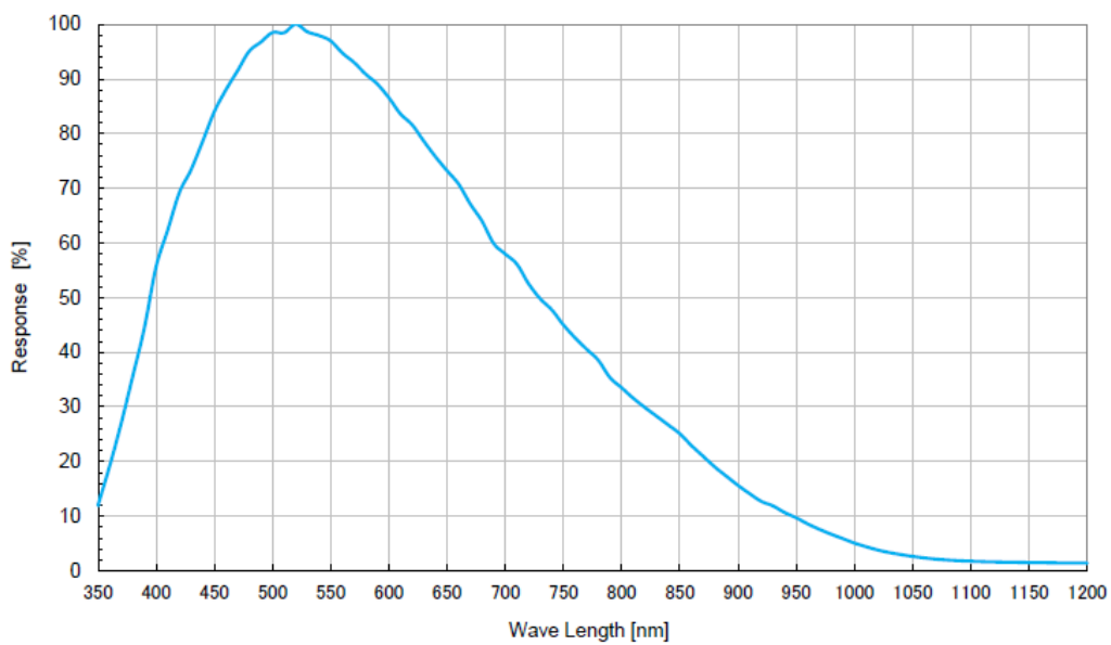
Figure 4-48 MER-201-25GM-P sensor spectral response
