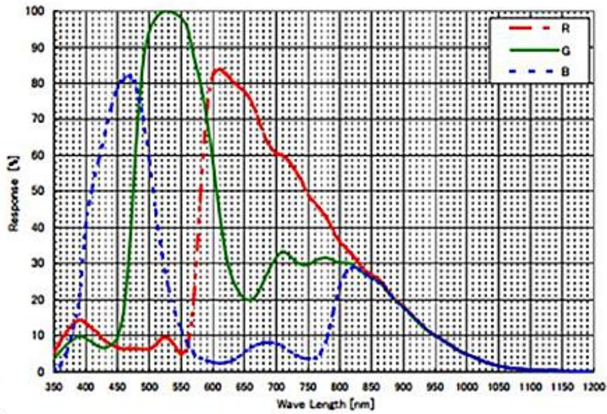
Figure 4-31 MER-132-43GC sensor spectral response
