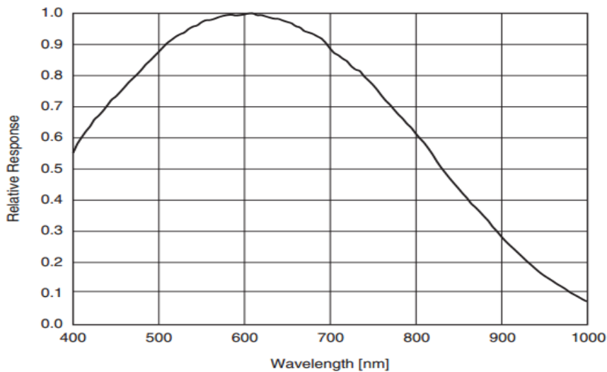
Figure 4-2 MER-030-120GM sensor spectral response
