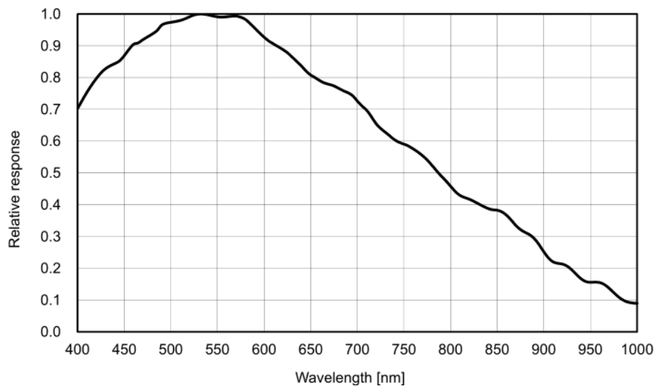
Figure 4-83 MER-2000-5GM sensor spectral response
