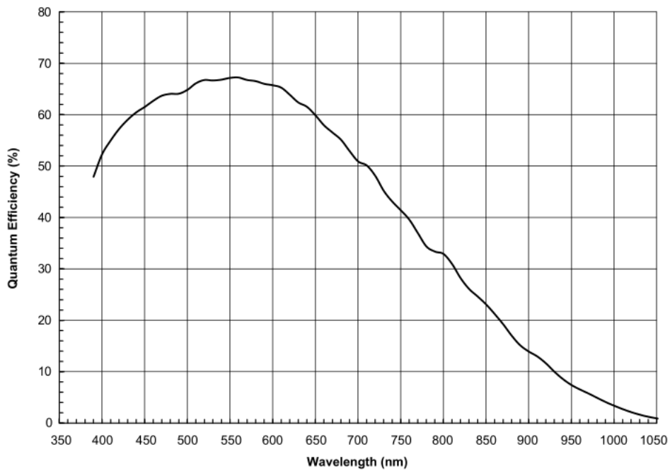
Figure 4-36 MER-133-54GM sensor spectral response
