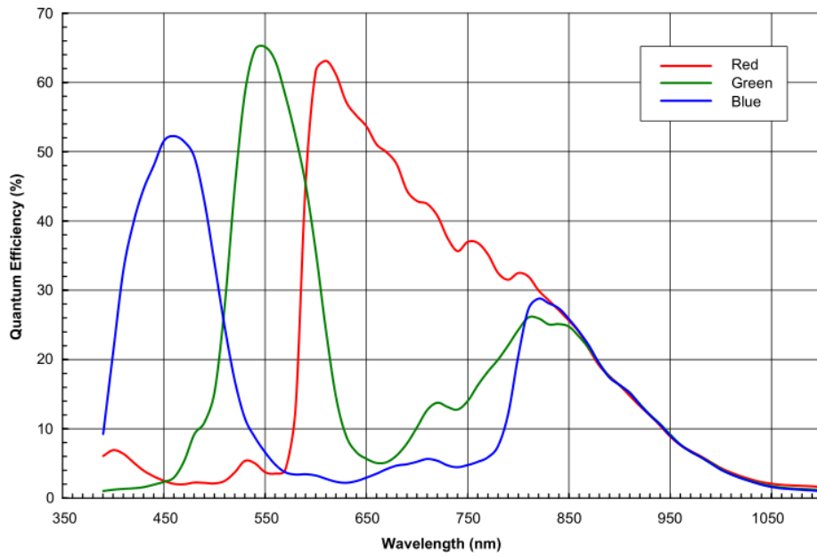
Figure 4-35 MER-133-54GC sensor spectral response
