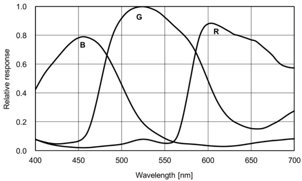
Figure 4-76 MER-1220-9GC sensor spectral response
