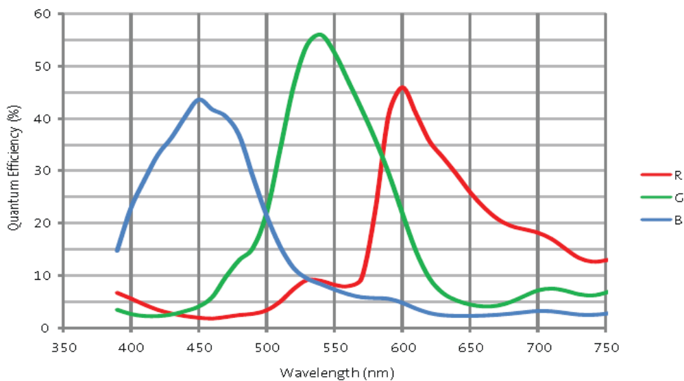
Figure 4-81 MER-1520-7GC-P sensor spectral response
