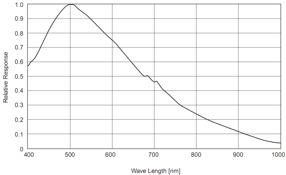
Figure 4-44 MER-200-20GM-P sensor spectral response
