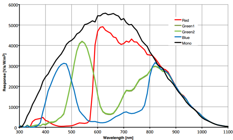
Figure 4-6 MER-031-300GC-P / MER-031-300GM-P sensor spectral response
