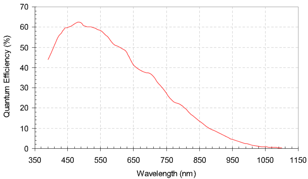
Figure 4-59 MER-500-14GM-P sensor spectral response
