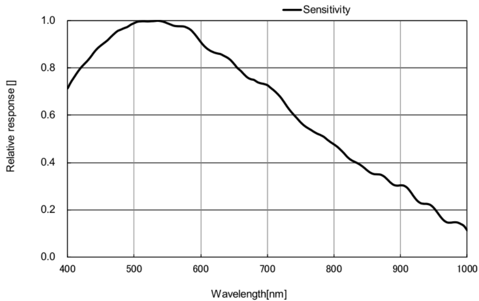
Figure 4-77 MER-1220-9GM sensor spectral response
