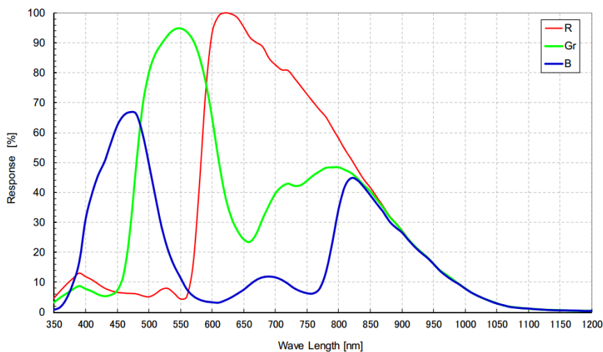
Figure 4-8 MER-032-120GC sensor spectral response
