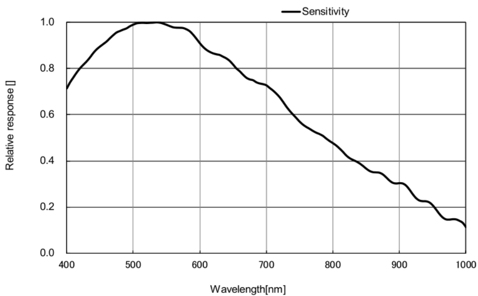
Figure 4-79 MER-1220-9GM-P sensor spectral response
