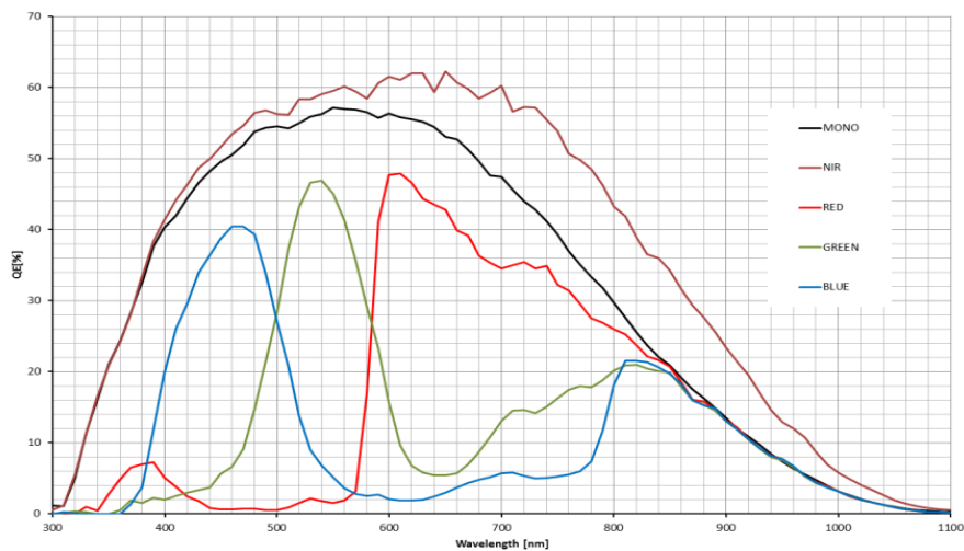
Figure 4-67 MER-531-20GC-P / MER-531-20GM-P sensor spectral response
