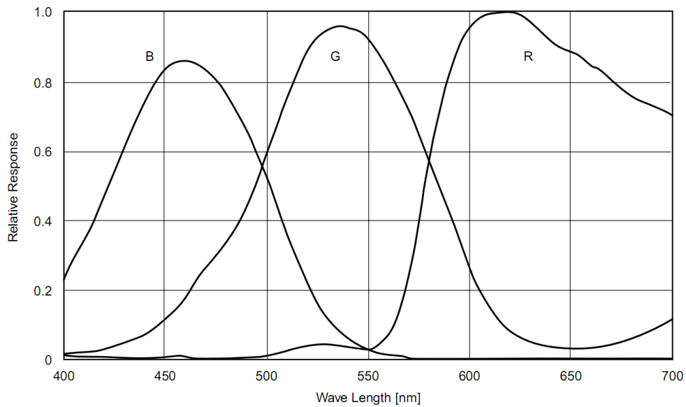
Figure 4-39 MER-200-14GC sensor spectral response
