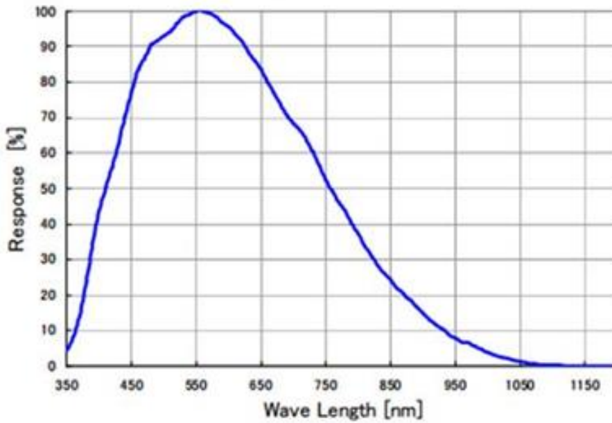
Figure 4-30 MER-132-30GM sensor spectral response
