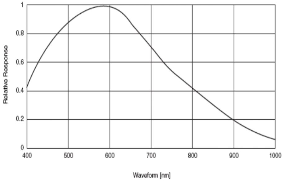
Figure 4-24 MER-125-30GM-P sensor spectral response
