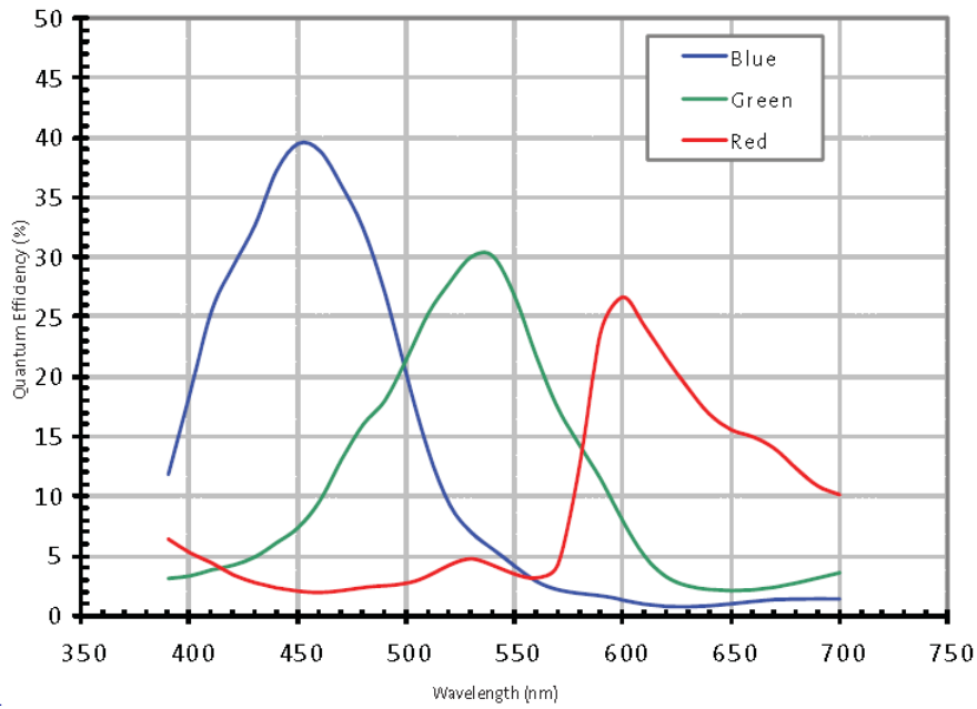
Figure 4-72 MER-1070-10GC sensor spectral response
