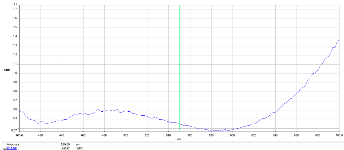
Figure 6-2 Transparent glass reflectance curve for MERCURY series mono camera
