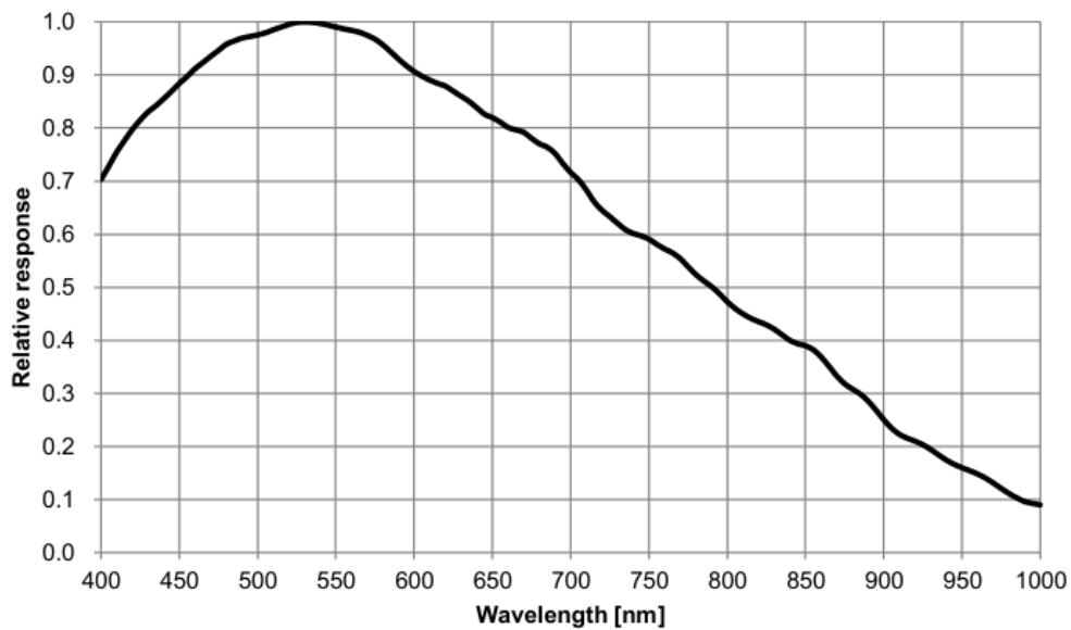
Figure 4-71 MER-630-16GM-P sensor spectral response
