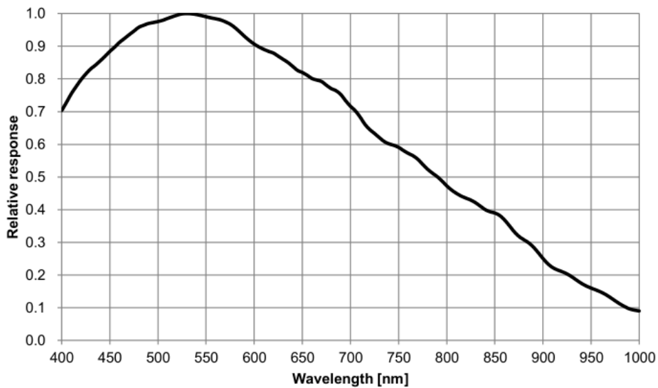
Figure 4-69 MER-630-16GM sensor spectral response
