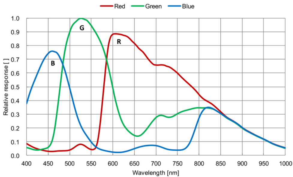
Figure 4-53 MER-231-41GC-P sensor spectral response
