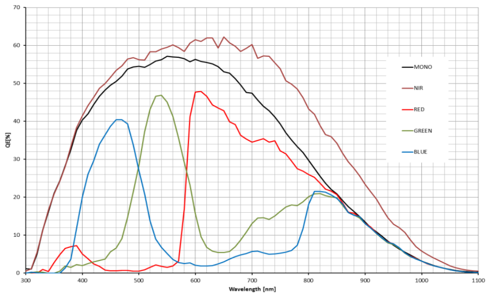
Figure 4-55 MER-232-48GM-P NIR sensor spectral response
