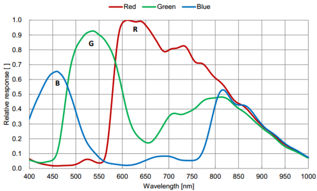
Figure 4-60 MER-503-20GC sensor spectral response
