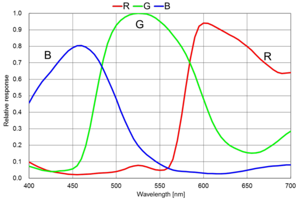
Figure 4-70 MER-630-16GC-P sensor spectral response
